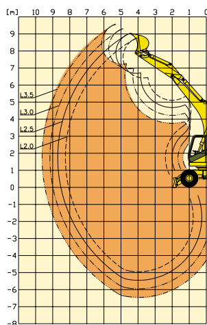
Monoblock M5.1
